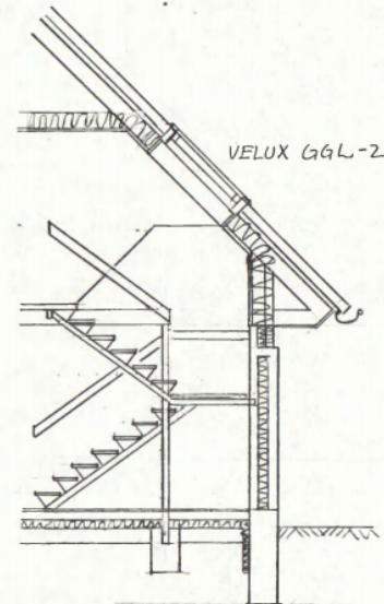
SNIT B
