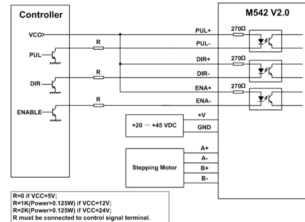
Figure 10: Typical connection
