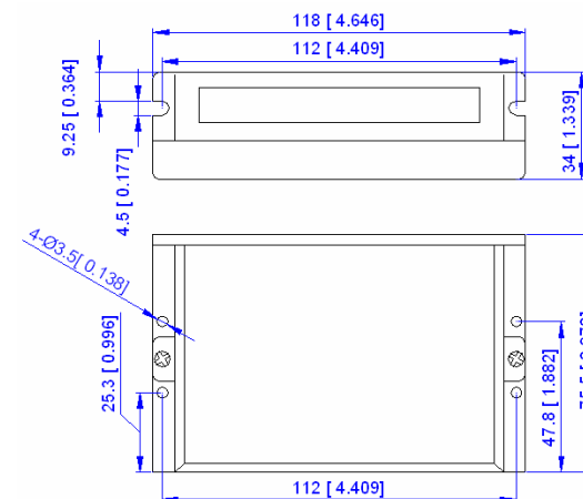
Figure 1: Mechanical specifications
