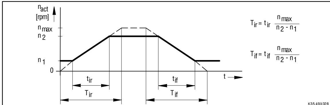
FIG 7-3 Calculation of the acceleration and deceleration times
